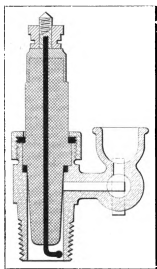
ALL-IN-ONE SPARK PLUG.
